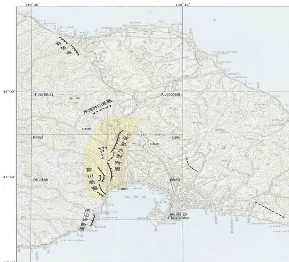
函館平野西縁断層帯の位置図 Location of Hakodate-heiya-seien Fault zone
