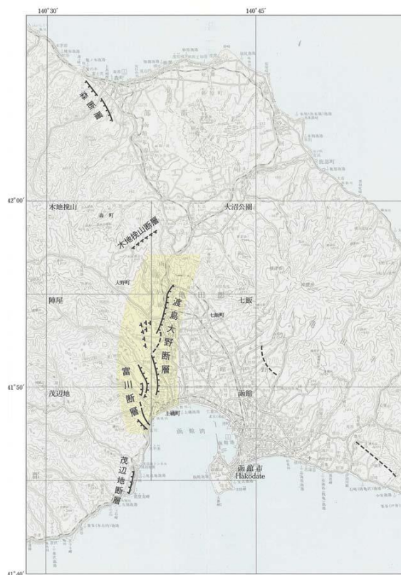
函館平野西縁断層帯の位置図 Location of Hakodate-heiryaseien Fault zone
